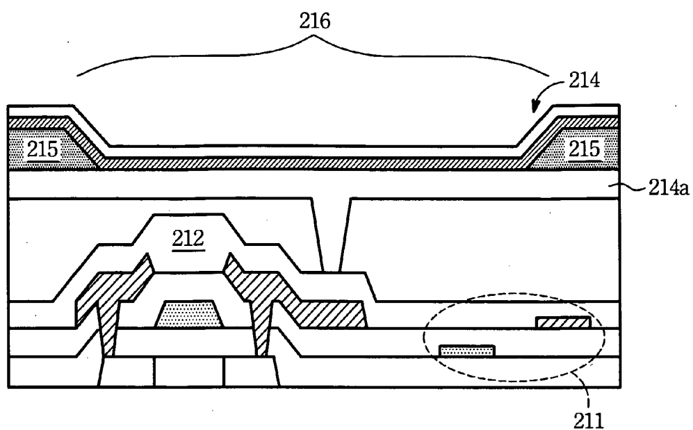
FIG. 1 C (Prior Art)
